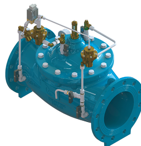
M3700 [DN300 a DN1000]
