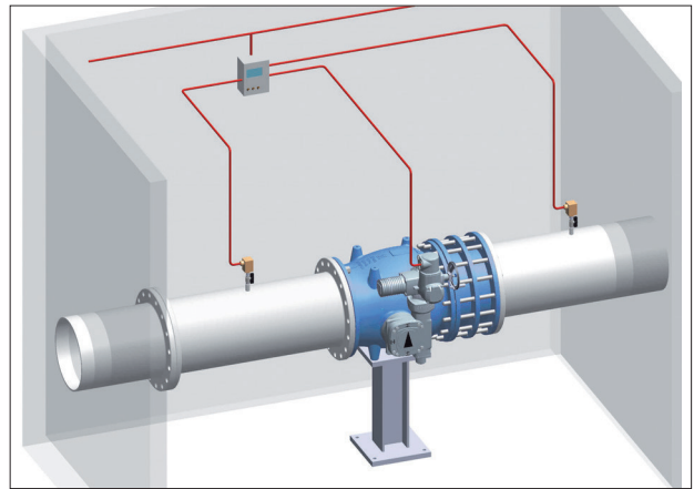
PRESSURE CONTROL CONFIGURATION
