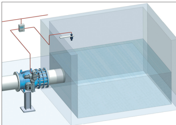
WITH ELECTRIC TYPE ACTUATOR AND LEVEL SENSOR
