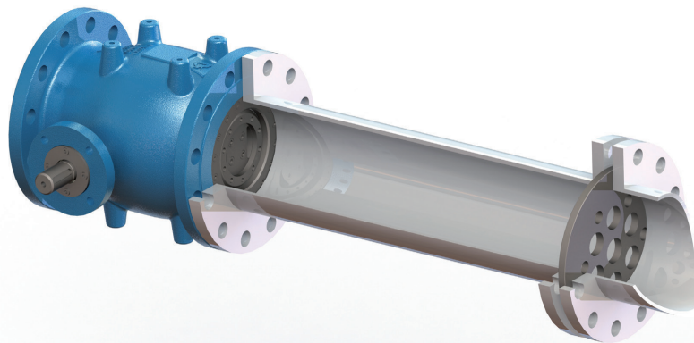
DISSIPATING PLATE
