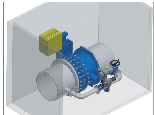
BY-PASS FOR FILLING LARGE PIPELINES
