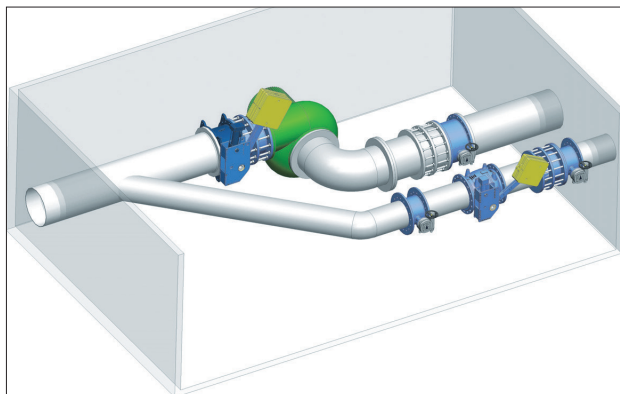
BY-PASS FOR TURBINE-GENERATOR
