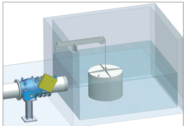
WITH COUNTERWEIGHT SYSTEM AND FLOAT
