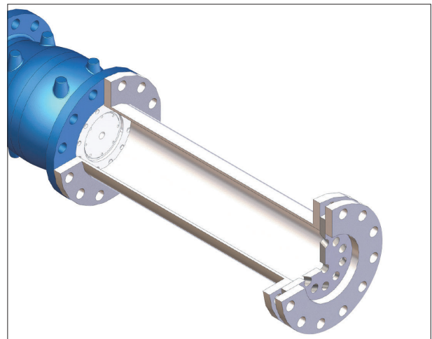
DISSIPATING PLATE - FREE DISCHARGE
