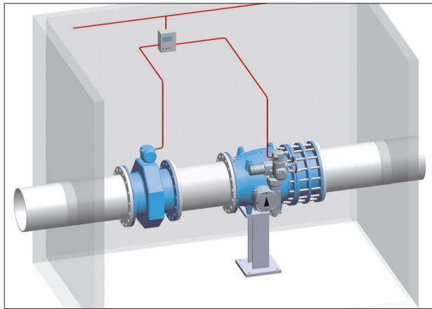
FLOW CONTROL CONFIGURATION
